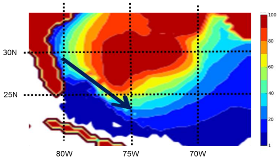
4 Figure 7. (Top) 120-h WW3_TC_OFCL ensemble forecasts of maximum significant 5 wave height, and (bottom) 0-120 h cumulative probabilities of 12-ft seas with 6 approximate El Faro route (blue arrow). Blue (red) shades indicate 0-40% (80-100%) 7 probabilities. (Lower right) NHC best track and estimated 12-ft seas radii. Initial time in 8 all panels is 00 UTC September 29, 2015.
