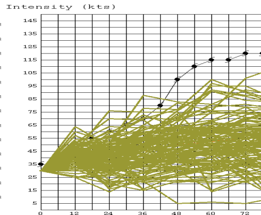
4 Figure 3. (Left) Ensemble forecast tracks and (right) forecast intensity (kt) out to 72 h 5 for GFS (top), NAVGEM (middle), and the WSP (bottom). Case is Joaquin (al12015) 6 on September 29 th , 2015. Ensemble forecasts are gold, NHC forecast is orange and 7 best track is black with the southernmost position being the 72-h verifying position.
