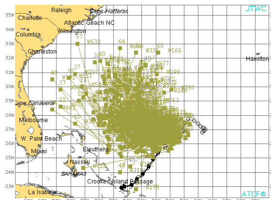
4 Figure 3. (Left) Ensemble forecast tracks and (right) forecast intensity (kt) out to 72 h 5 for GFS (top), NAVGEM (middle), and the WSP (bottom). Case is Joaquin (al12015) 6 on September 29 th , 2015. Ensemble forecasts are gold, NHC forecast is orange and 7 best track is black with the southernmost position being the 72-h verifying position.
